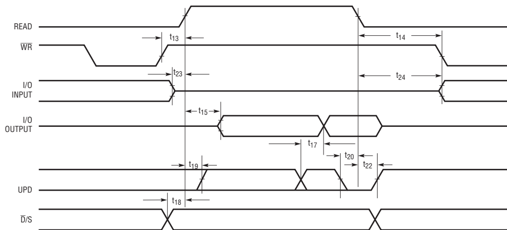
Readback Timing
